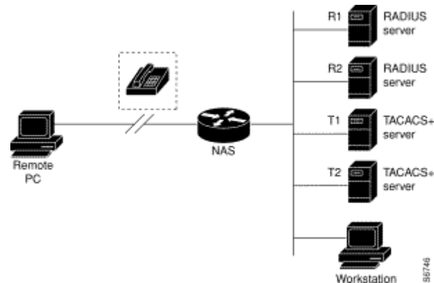
Figure 0-1 Typical AAA Network Configuration
